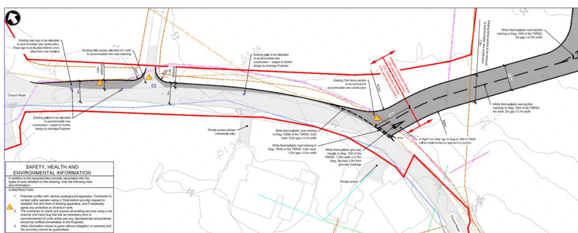
Figure 3.3 Church Road Staff Access Junction
