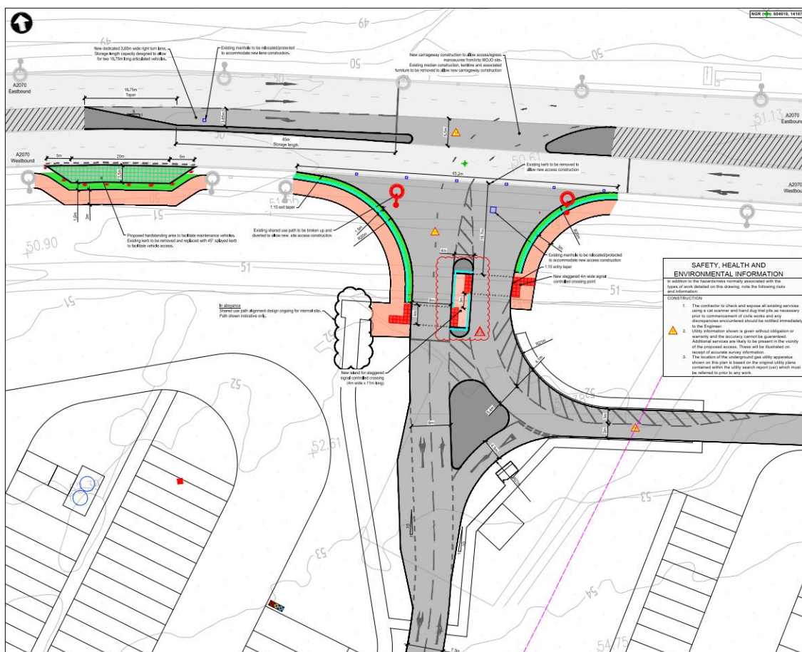
Figure 3.2: Permanent Site Access General Arrangement
